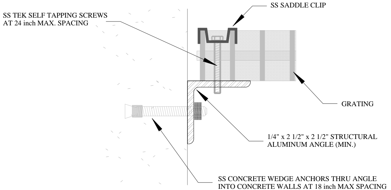
SECTION VIEW
